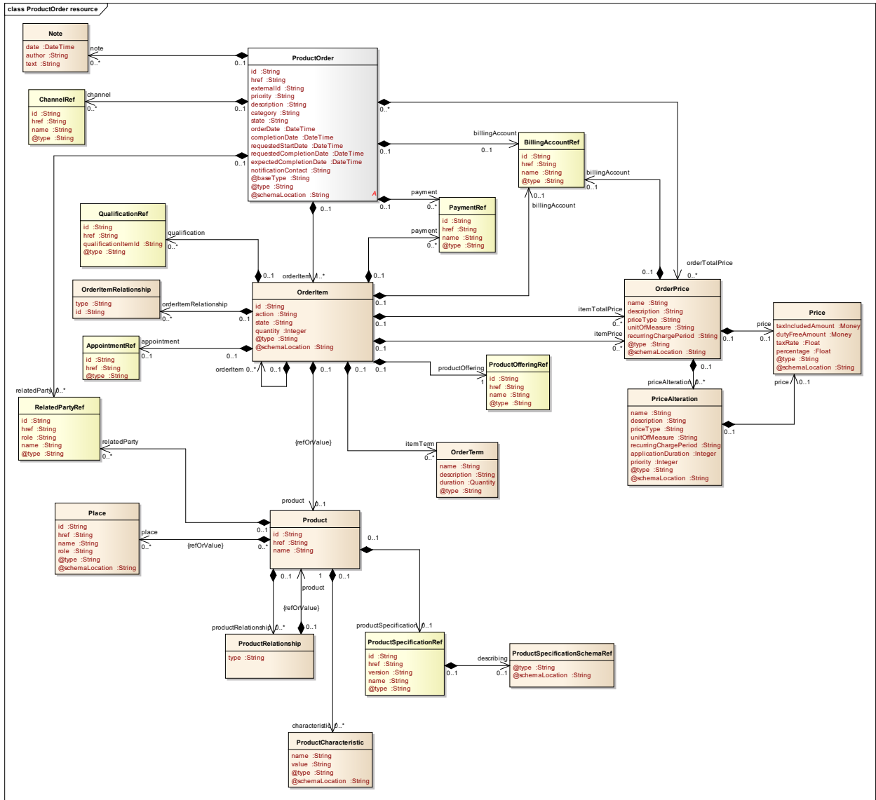
Figure 1. RefOrValue annotation used in API Data model
