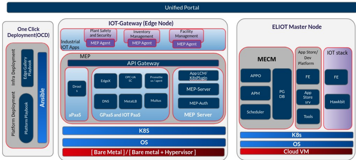
Figure 2: Software Architecture
