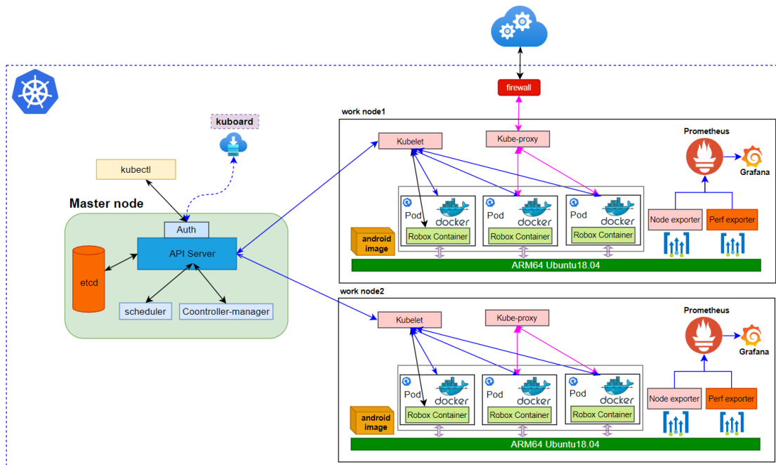
Robox Deployment Framework
